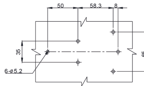
Panel Cutout
