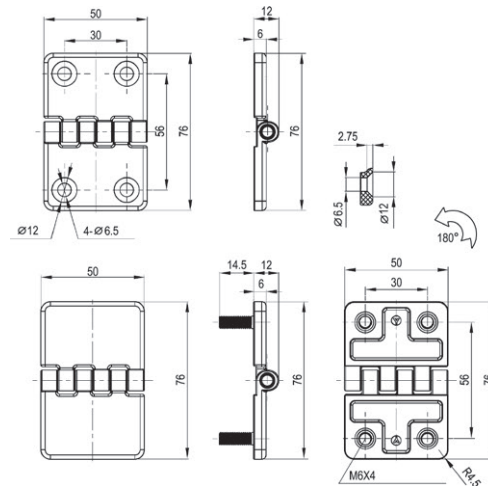
Countersunk Screw M6
