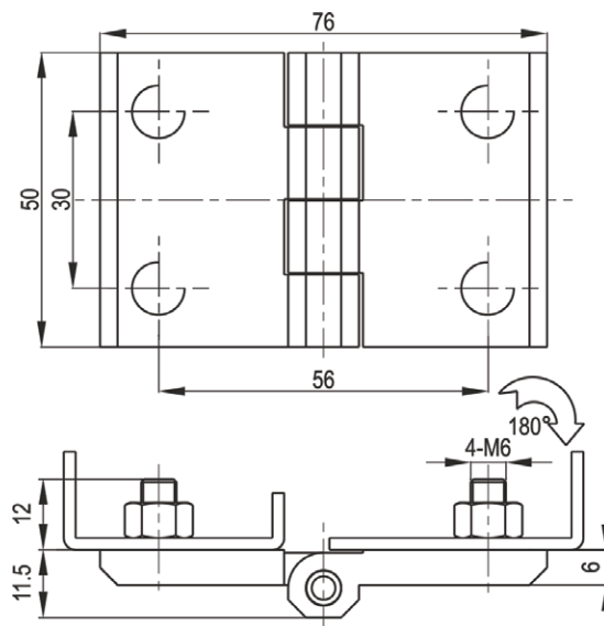
With Threaded Studs M6
