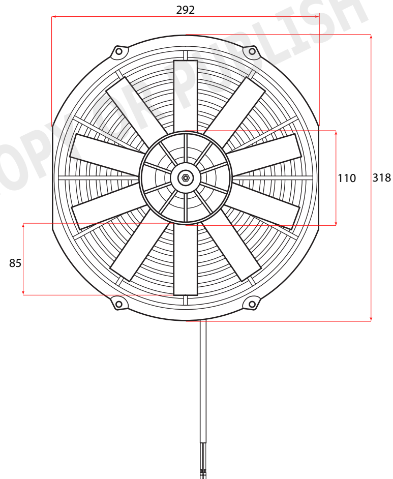
REAR VIEW
