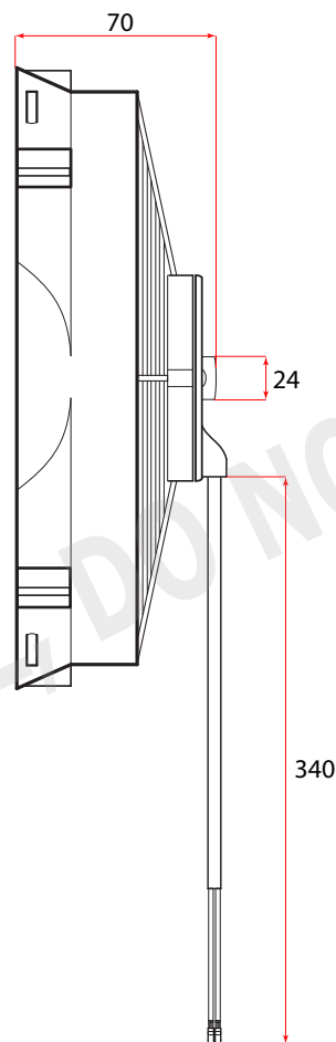
SIDE VIEW
