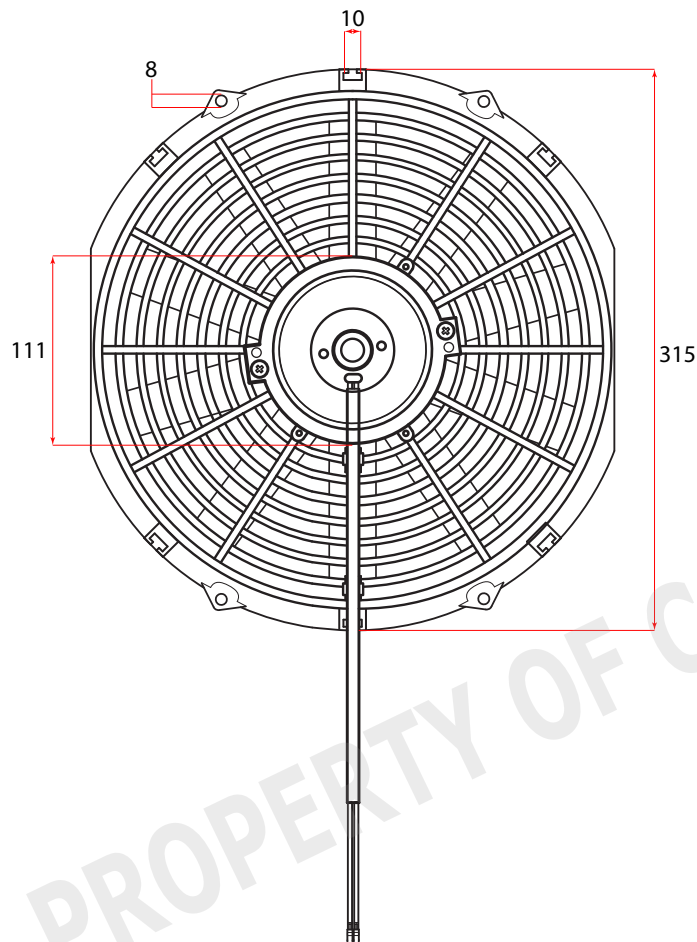
FRONT VIEW
