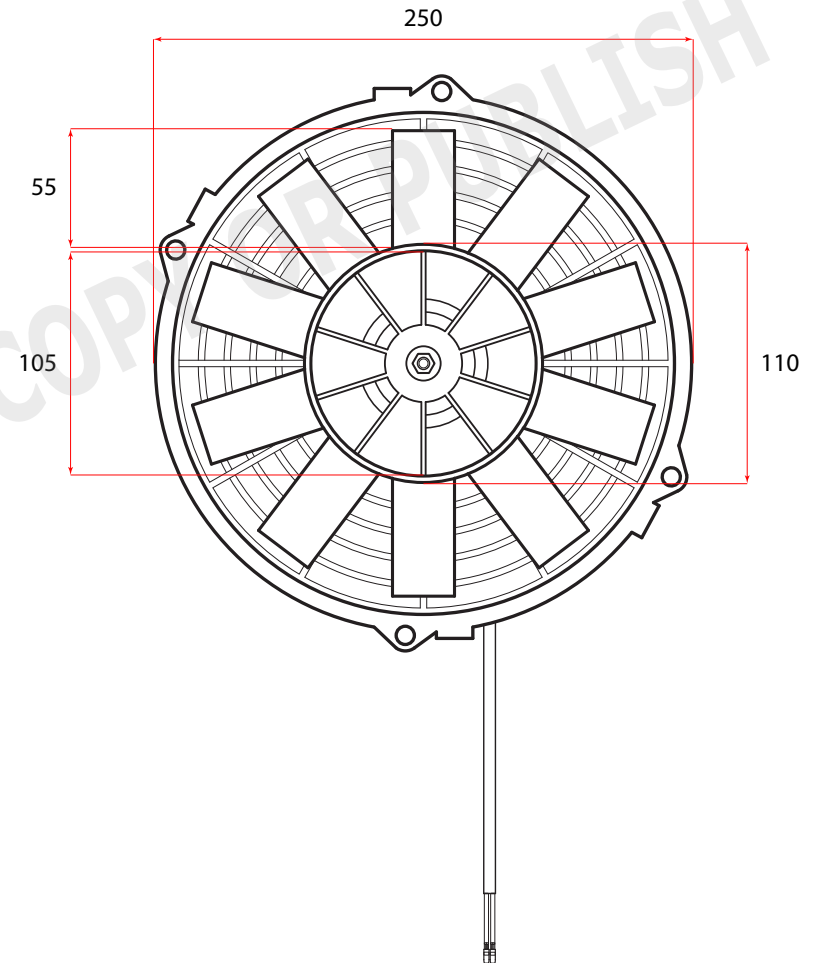
REAR VIEW
