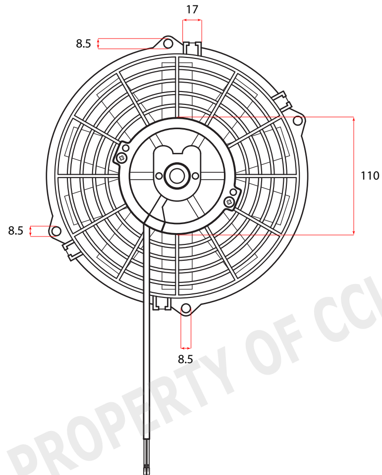
FRONT VIEW
