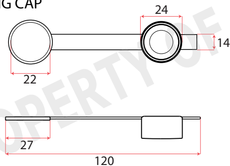
COVERING CAP
