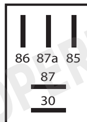
PIN LAYOUT
