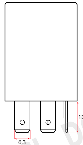
PIN LAYOUT
