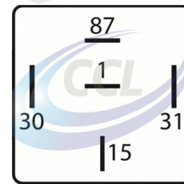
PIN LAYOUT
