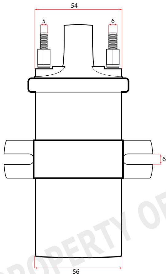
FRONT VIEW
