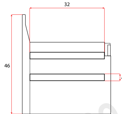
METAL TERMINALS
