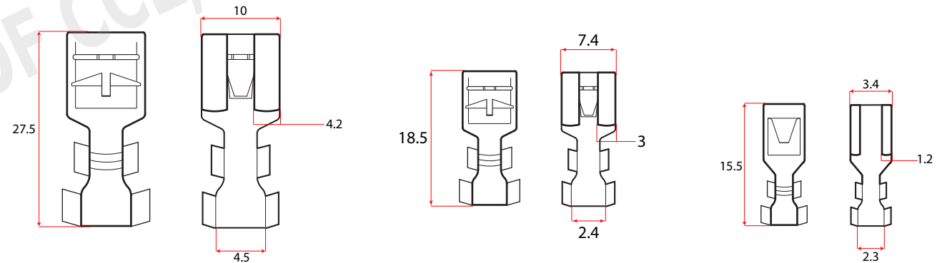
METAL TERMINALS
