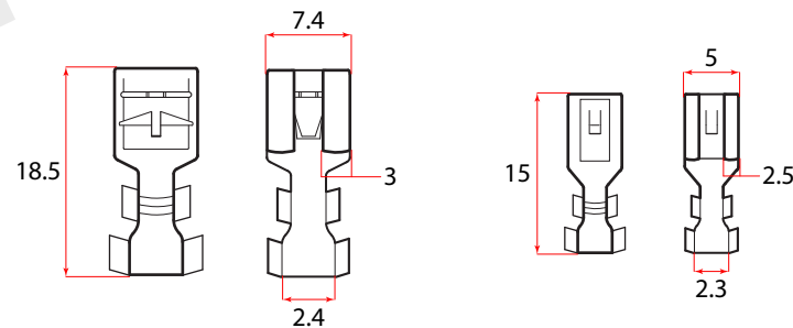
METAL TERMINALS
