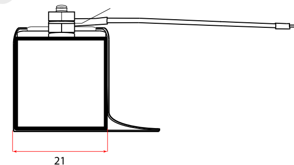
SIDE VIEW 2
