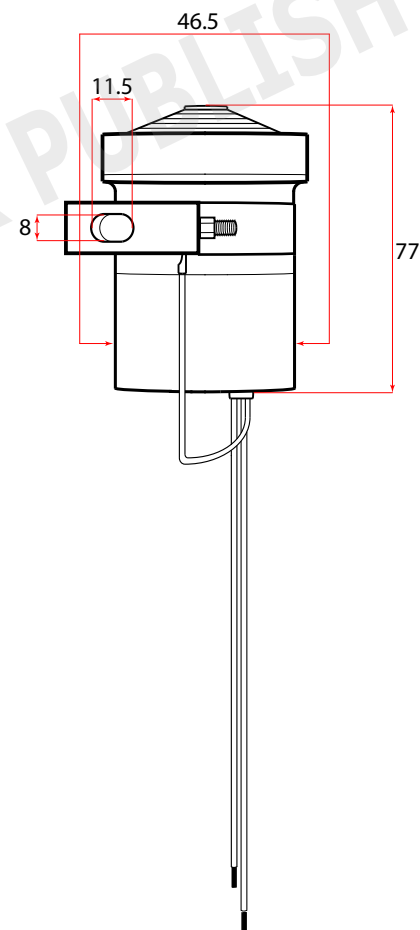
SIDE VIEW 2
