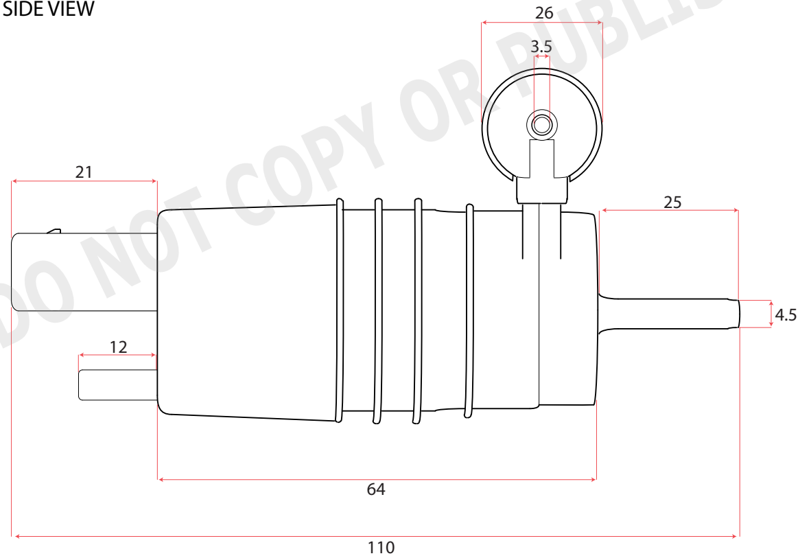
SIDE VIEW
