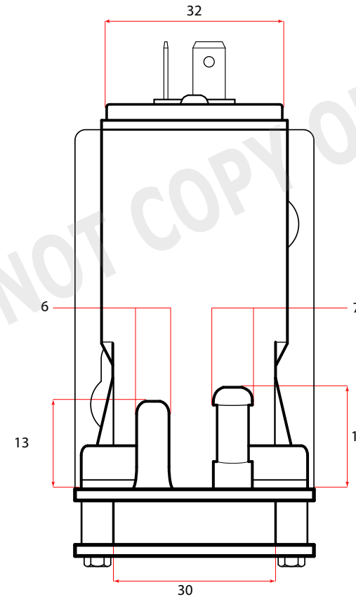
BOTTOM VIEW
