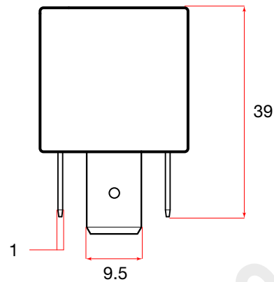
PIN LAYOUT
