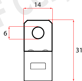
METAL BRACKET
