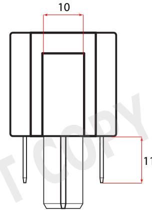
SIDE VIEW 2
