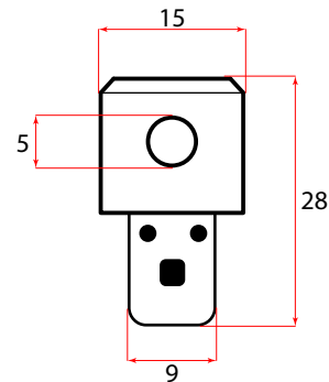
METAL BRACKET
